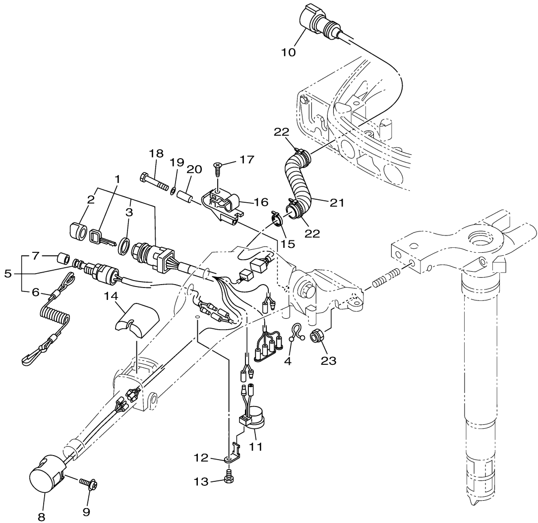
6X4 TILLER HANDLE KIT (F25A)
